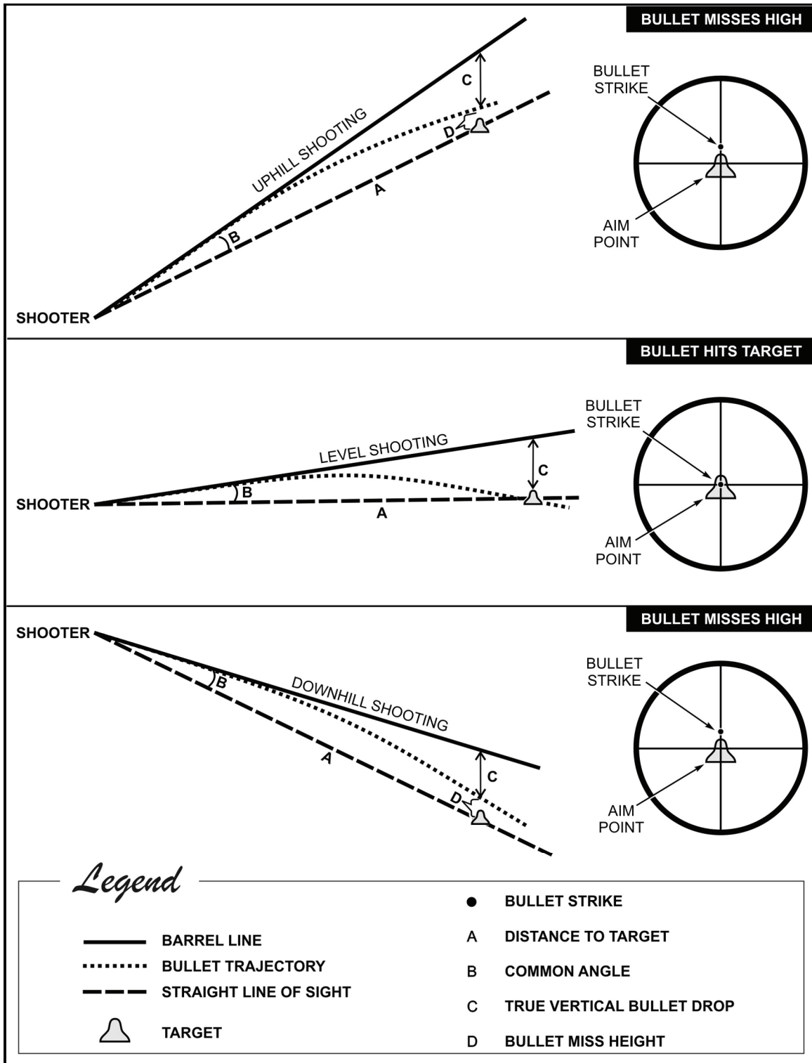
Figure 6-1. Angle shooting
