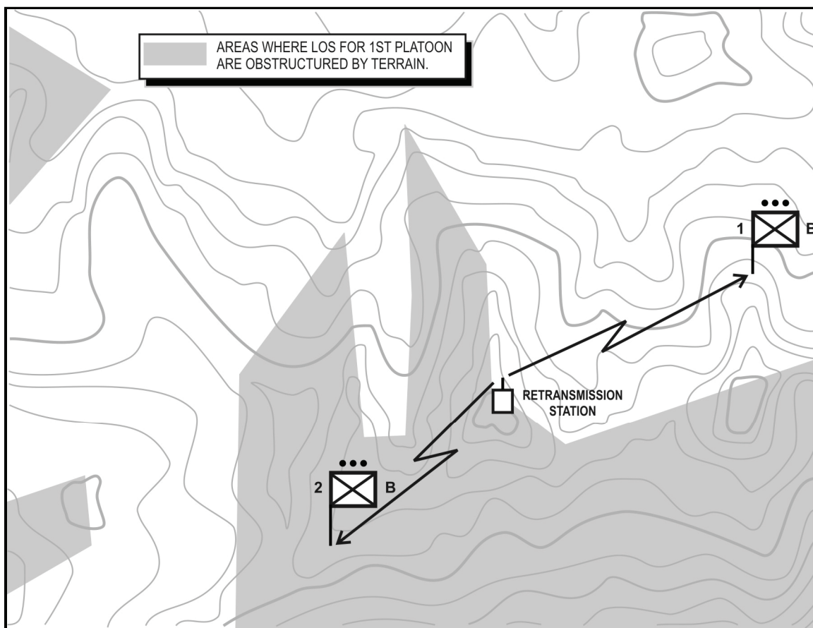
Figure 2-1. Retransmission station
