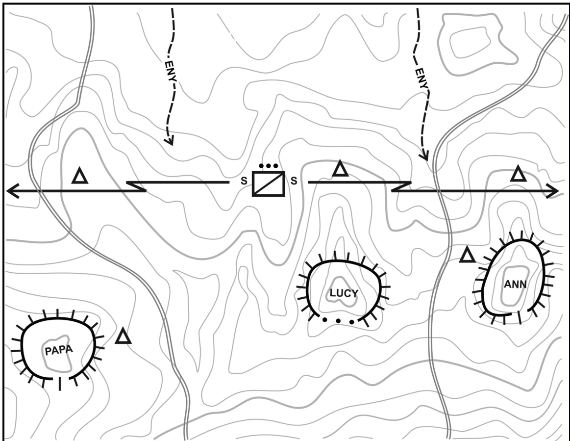
Figure 5-10. Combat outposts
